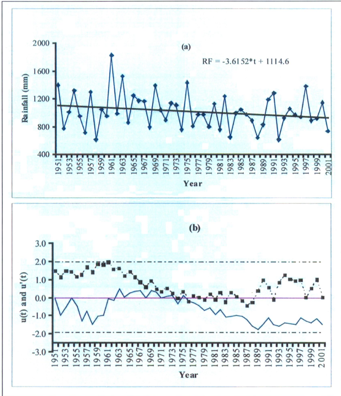
Figure 3: Temporal variability of (a) annual rainfall and (b) u(t) and u'(t) for annual rainfall
