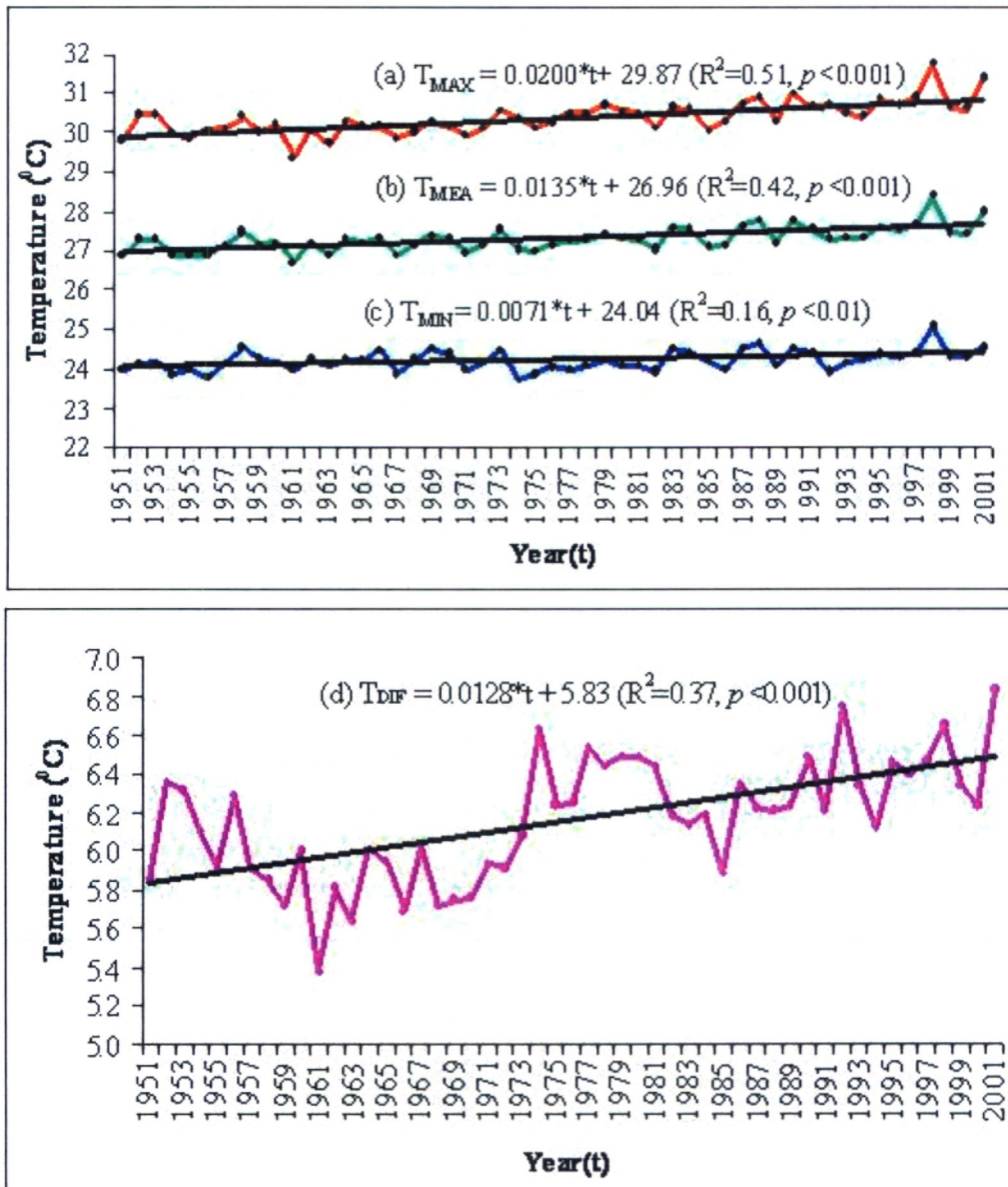
Figure 1: Annual variability of T_{MAX} , T_{MEA} , T_{MIN} and T_{DIF} along with the corresponding trend line
