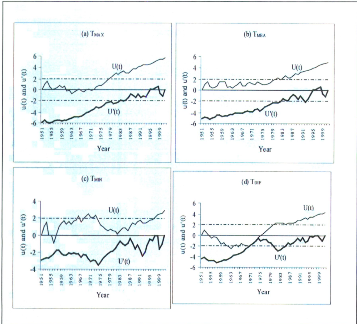
Figure 2: Temporal patterns of the trends in annual T_{MAX} , T_{MIN} , T_{MEA} and T_{DIF} temperature series and sequential values of the statistics u(t) and u'(t) of the M-K test with critical value of \pm 1.96 at the 5% level of significance
