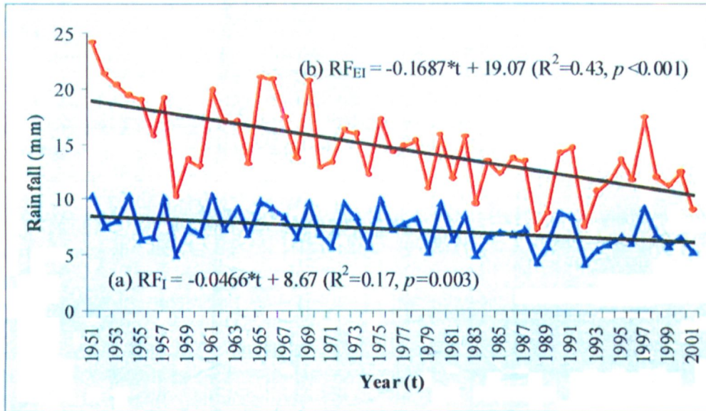
Figure 4: Temporal variability of (a) rainfall intensity and (b) effective rainfall intensity along with corresponding trend line
