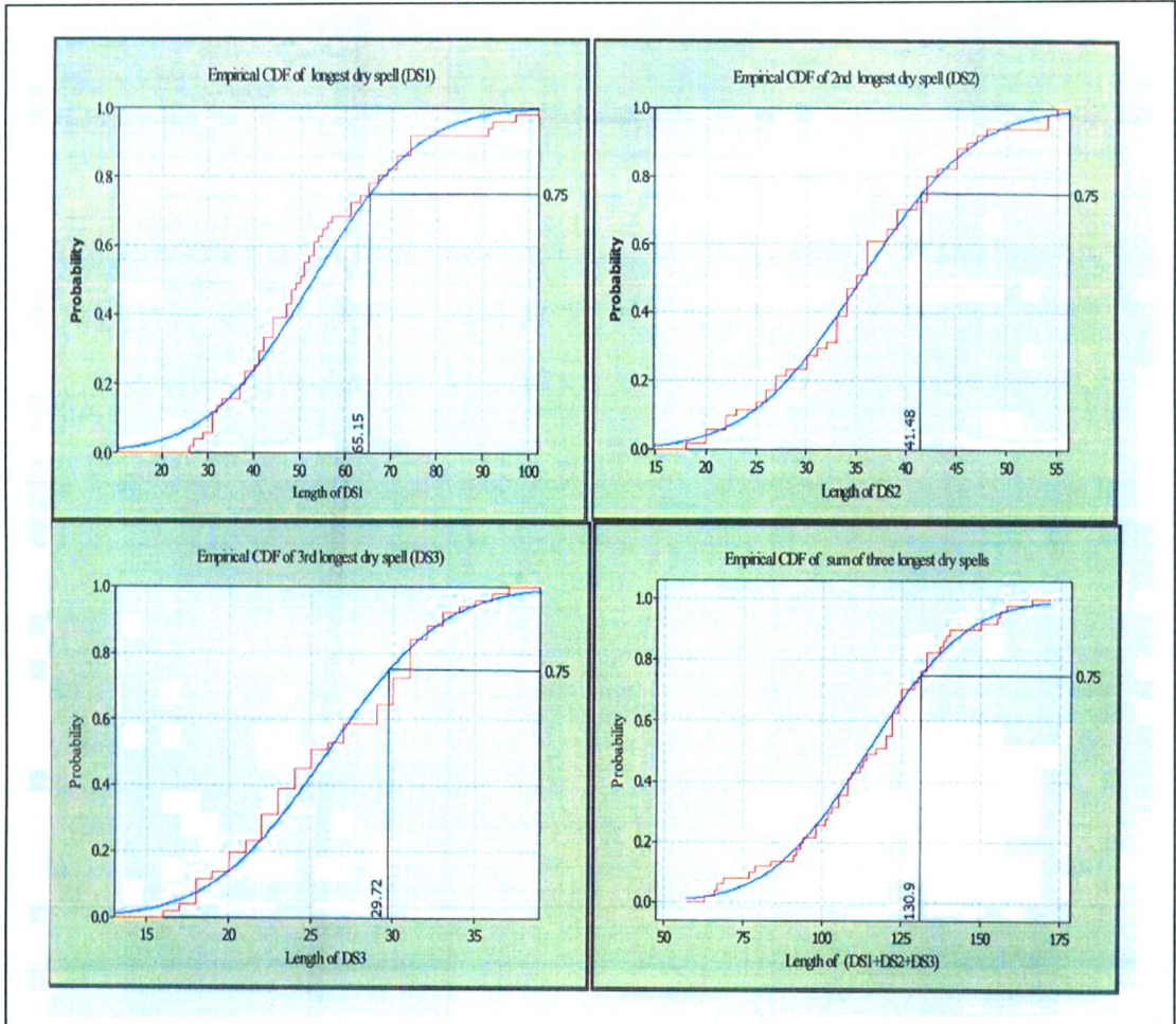
Figure 5: Empirical cumulative density function of (a) longest spell (DS1), (b) second longest dry spell (DS2), (c) third longest dry spell (DS3) and (d) sum of the three longest dry spells
